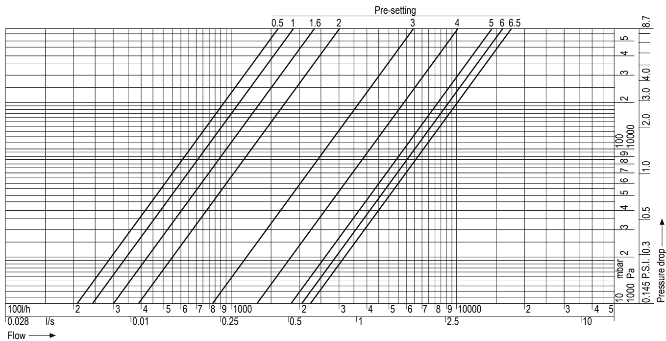
Flow Data V5032...B (DN40)
