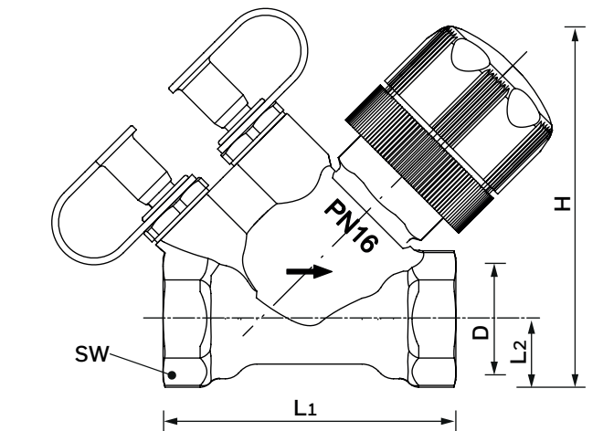
V5032...BLF Kombi-2-plus (DN15)
