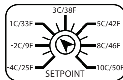
Figure 8 Setpoint Adjustment
