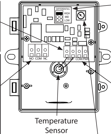
Figure 8 Setpoint Adjustment
