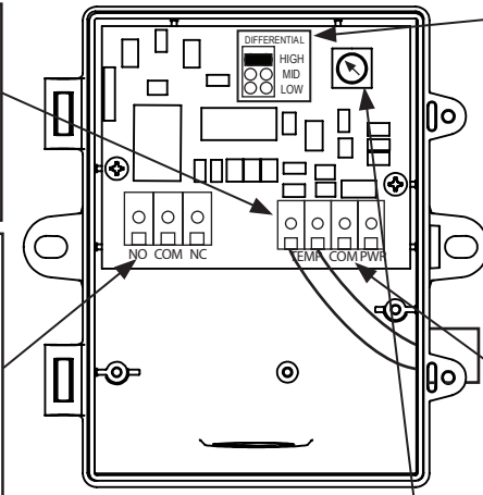
Figure 9 Setpoint Differential Setting
